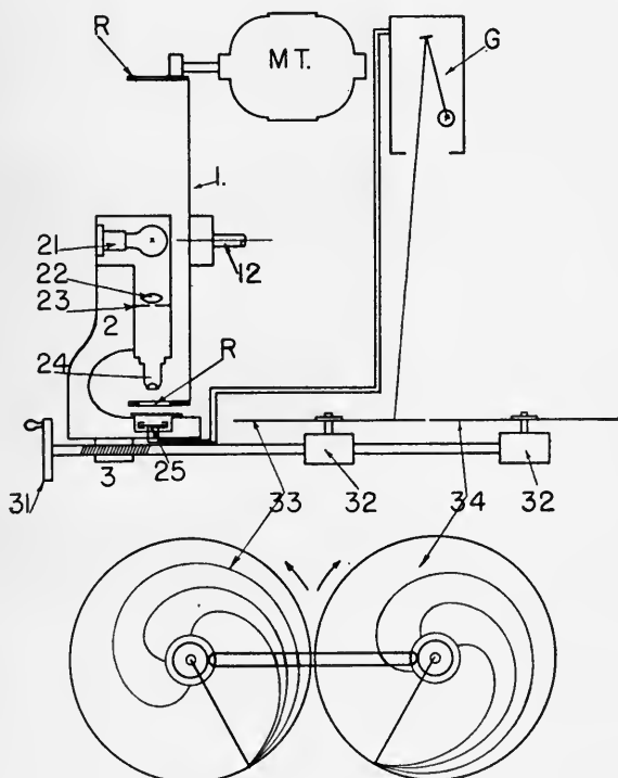
FIG. 7. Scheme of the graininess indicator. (The lower section shows a front view, on a larger scale, of the dials with three G -spirals on each.)
